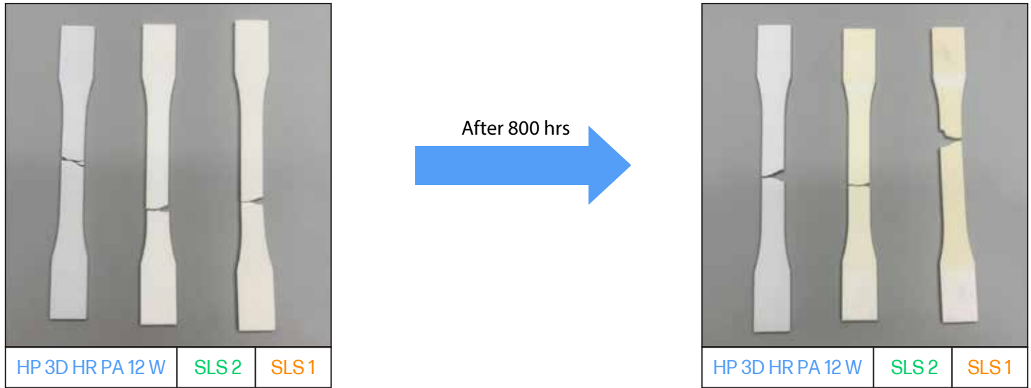
Figure 1: Each picture from left to right: HP 3D HR PA 12 W, SLS 2, and SLS 1.
