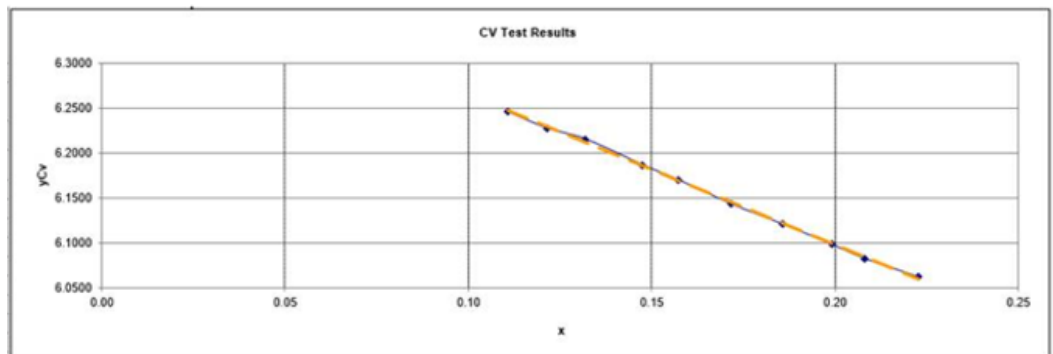
Completed choke valves flow tested at IMI Critical's facility.
