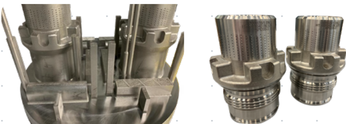
Image (Left) Two choke valves, optimized with IMI's DRAG technology, shown on the build plate after being 3D printed with Velo3D's Sapphire® system, and (Right) the two valves after finishing.
